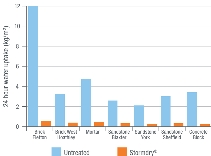
Effectiveness of Stormdry® on Different Substrates
