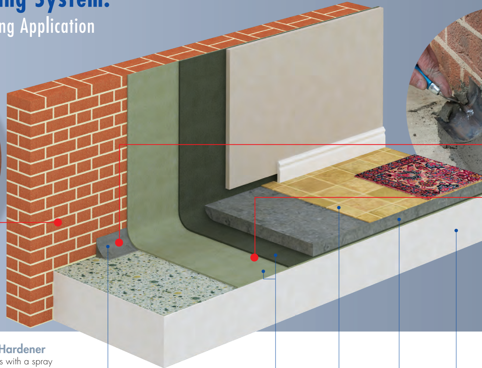
Vandex Unimortar 1 Fillet
