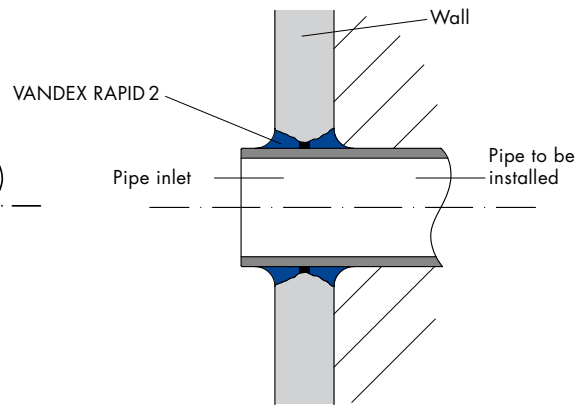
Detail Pipe Inlet
