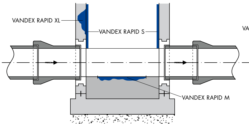
Cross Section Manhole
