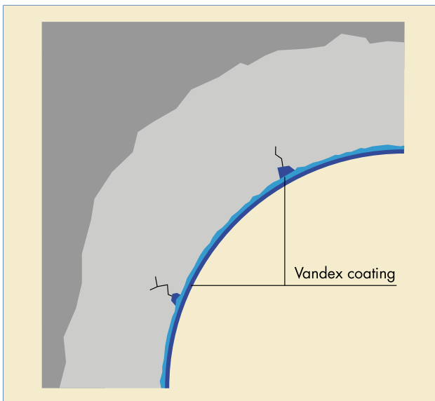
Internal waterproofing of a tunnel
