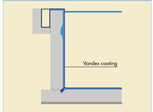
Swimming pool refurbishment
