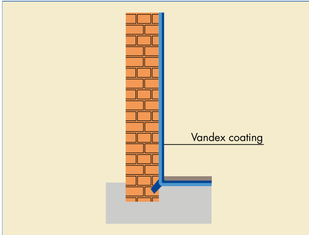
Basement waterproofing
