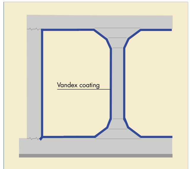
Tanking of a drinking water reservoir
