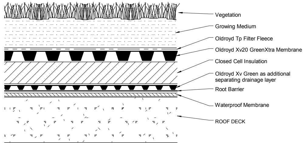
1. INVERTED ROOF
