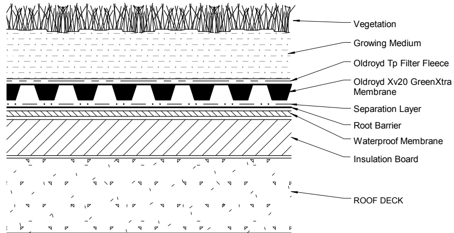
2. WARM ROOF
