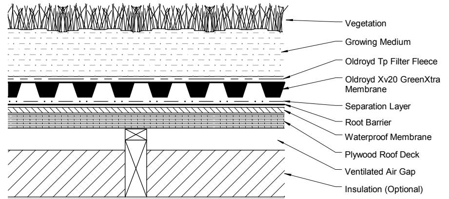
3. COLD ROOF
