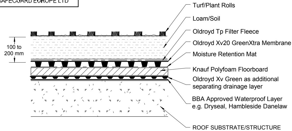
1. ROOF GARDEN / GREEN ROOF
