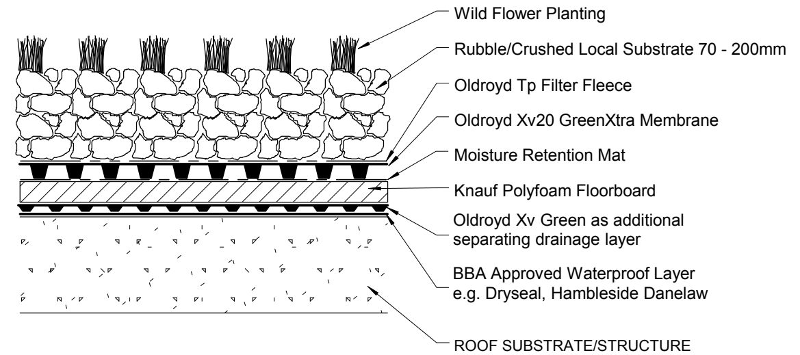
2. BROWN ROOF - For Biodiversity
