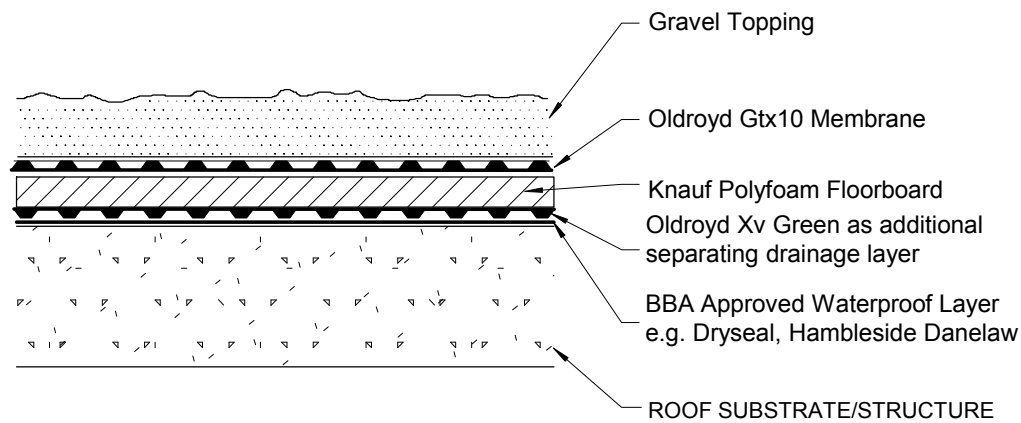
3. PROTECTED MEMBRANE ROOF
