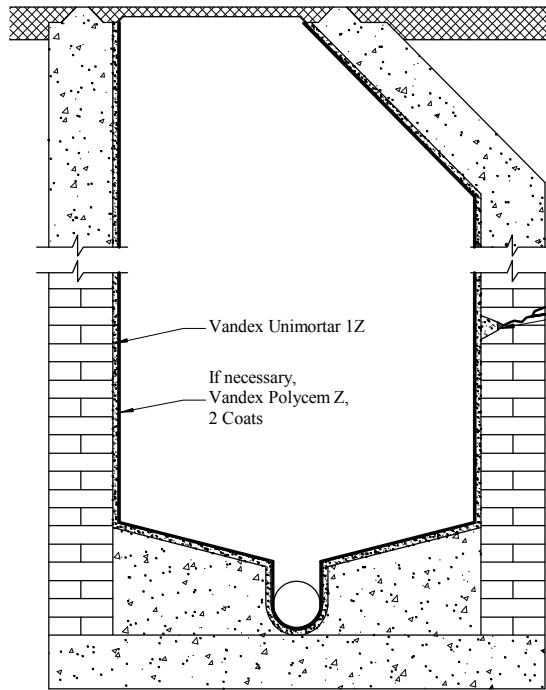
Masonry or Concrete Manhole Refurbishment
