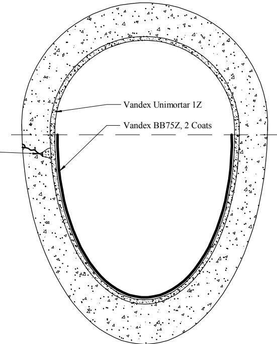
Concrete Pipe Refurbishment
