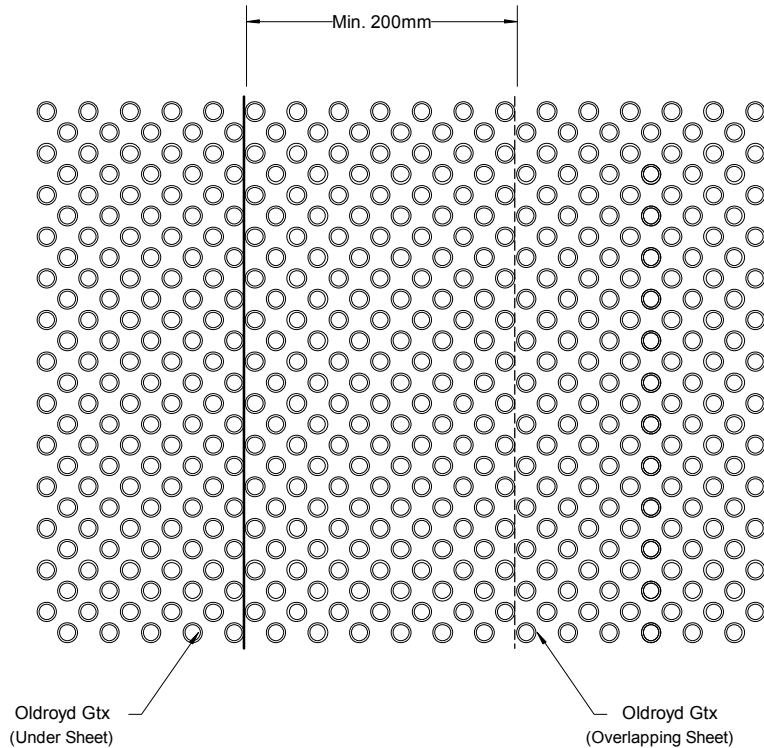
Vertical Joint Detail
